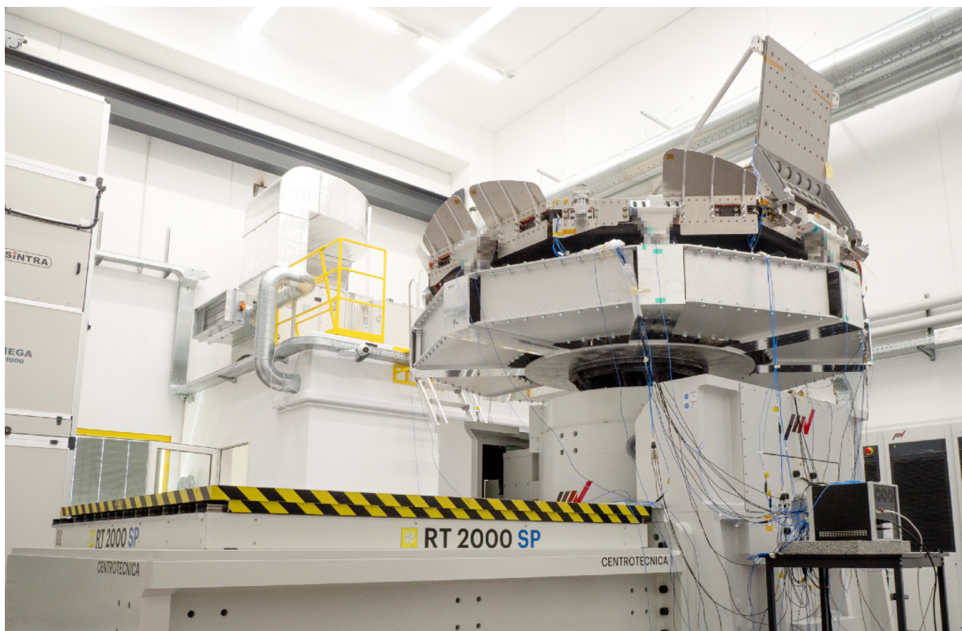
The AMS-02 COLLABORATION's antimatter analyzer to be mounted on the ISS. DUT on 200kN shaker in ISO 8 clean room.
